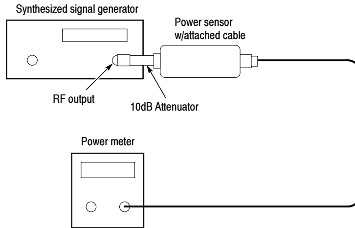
Figure 2-27: Power-reference hookup
