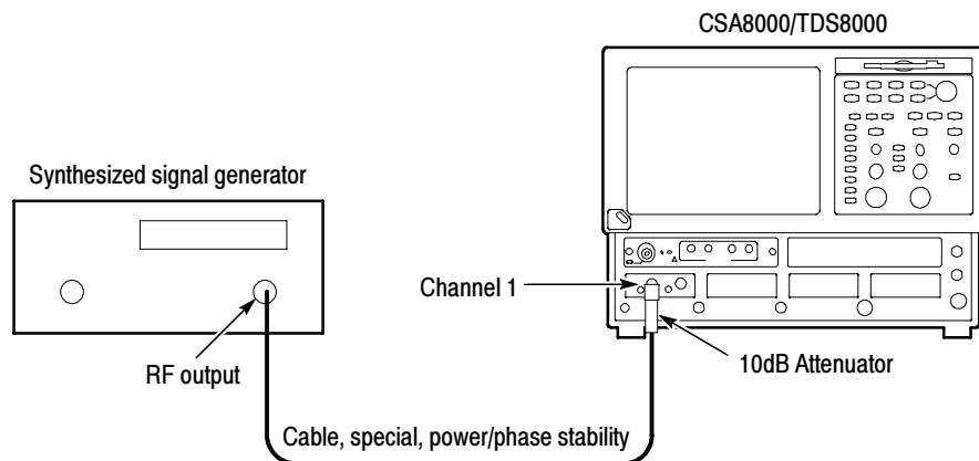
Figure 2-30: 80E01 reference signals hookup
