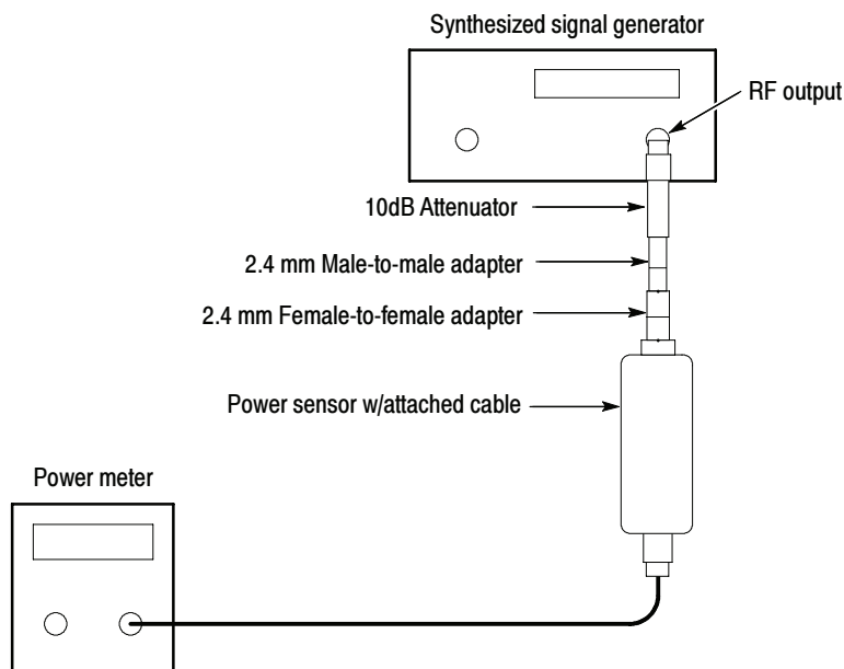
Figure 2-28: Adapter characterization hookup
