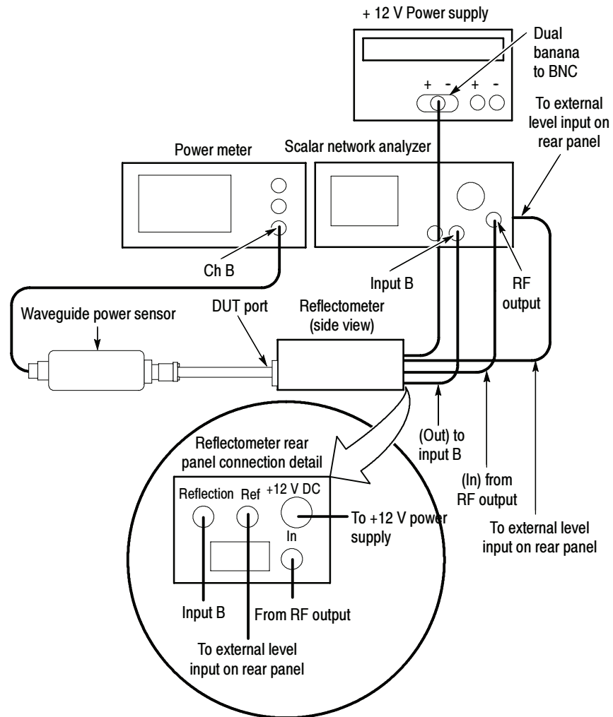
Figure 2-39: Hookup to measure Power-in
