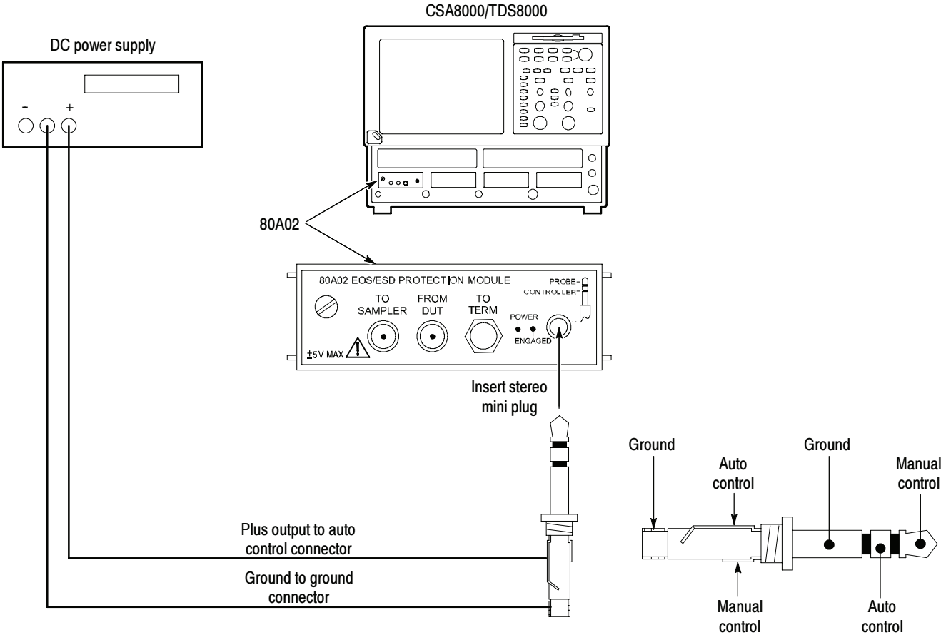
Figure 2-55: 80A02 test hookup
