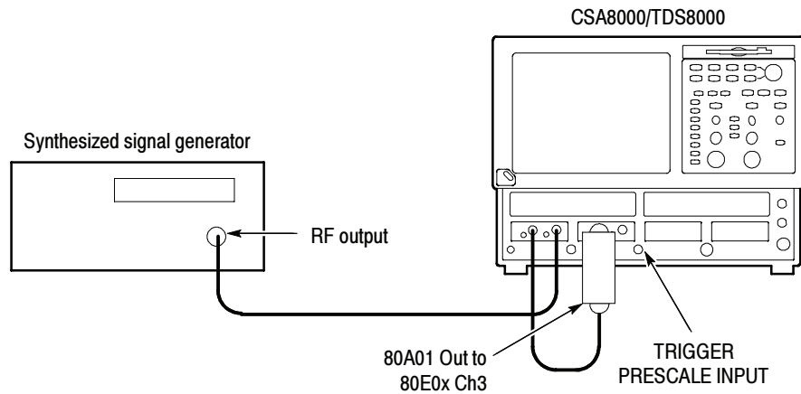
Figure 2-54: 80A01 test hookup
