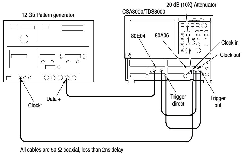
Figure 2-59: Hookup for Supported Clock Rates, Minimum Input Sensitivity, and Maximum Jitter Checks
