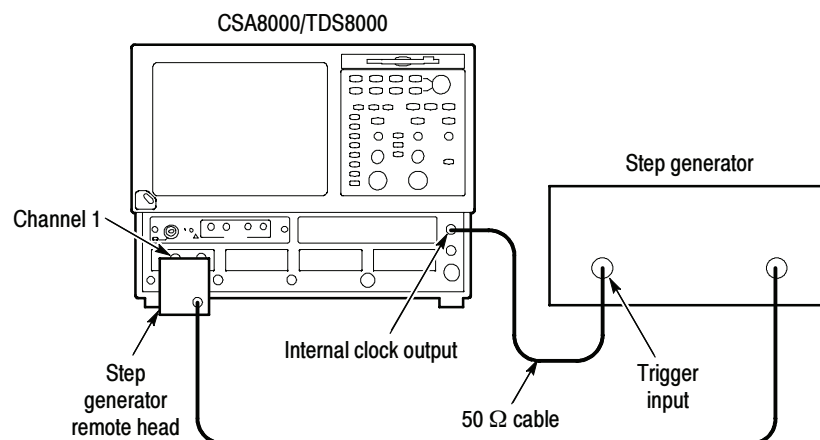
Figure 2-26: Rise Time hookup
