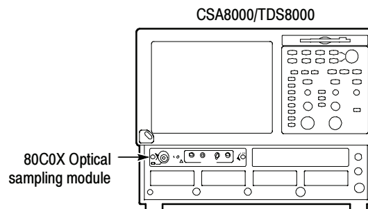
Figure 2-44: Dark level and vertical equivalent optical noise test hookup
