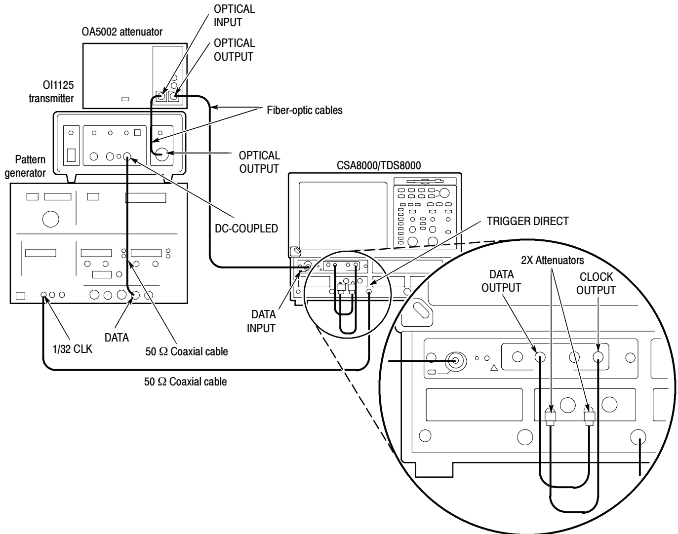
Figure 2-50: Clock recovery optical sensitivity range and recovered clock timing jitter hookup
