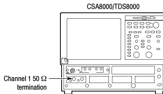
Figure 2-43: TDR system step response aberrations hookup
