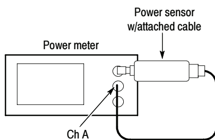
Figure 2- 32: Power-reference characterization hookup
