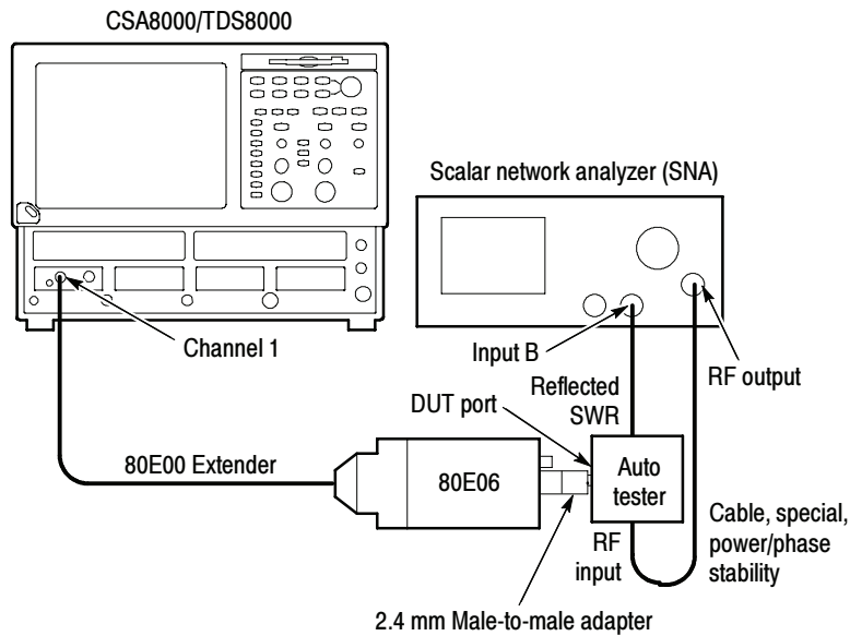
Figure 2- 36: 80E06 HF response hookup
