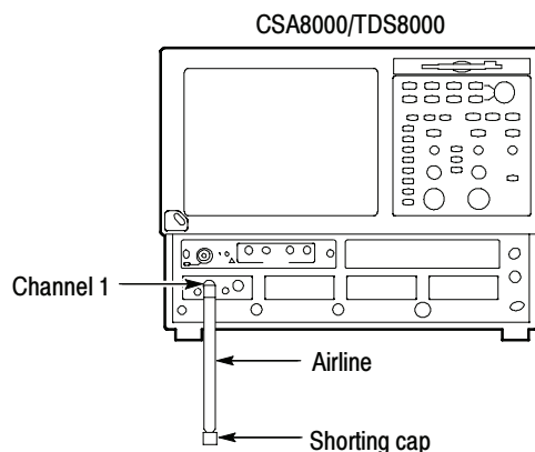
Figure 2- 42: TDR reflected rise time hookup
