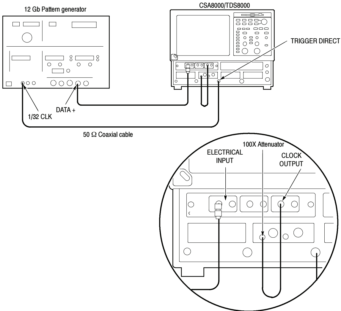
Figure 2-56: Clock recovery sensitivity range and recovered clock timing jitter hookup
