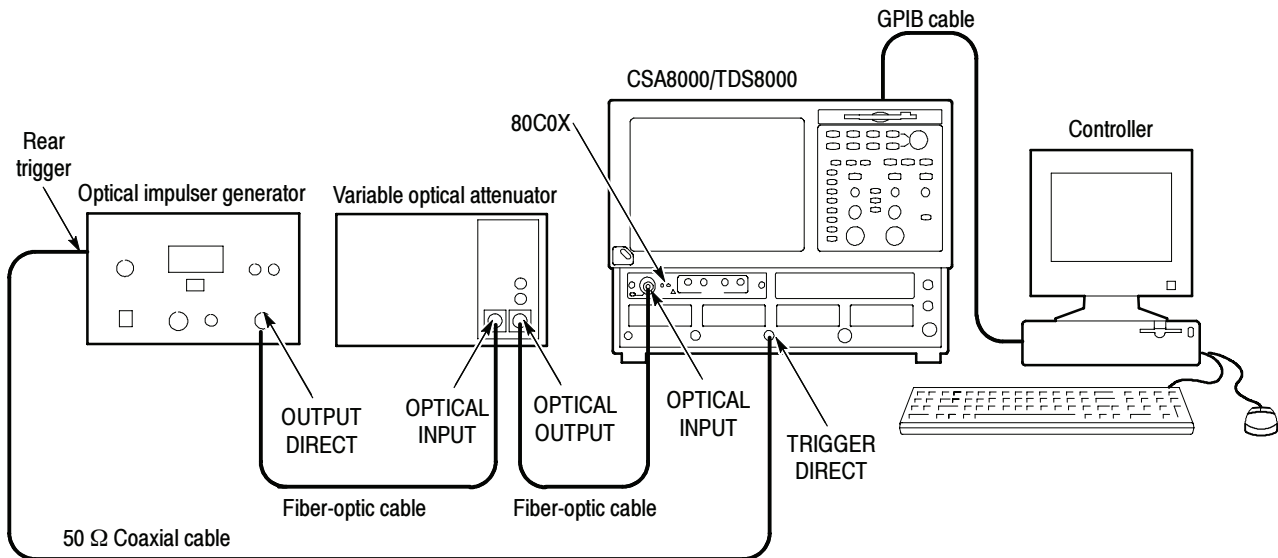
Figure 2-49: Integrated rise time and aberrations hookup
