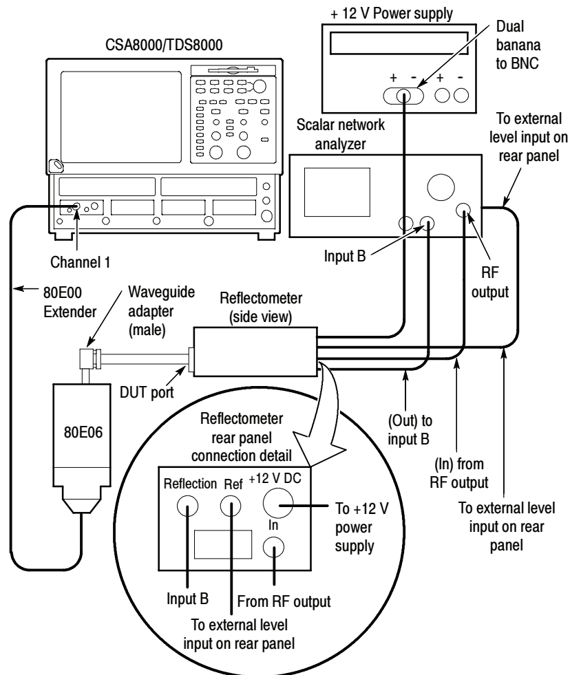
Figure 2-41: 80E06 HF response hookup
