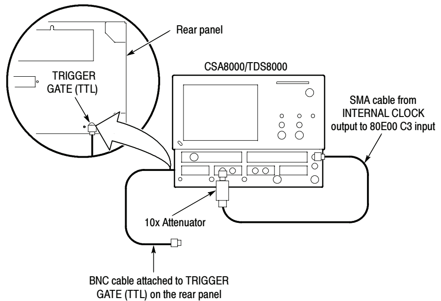
Figure 2-10: Hookup for the gated trigger tests
