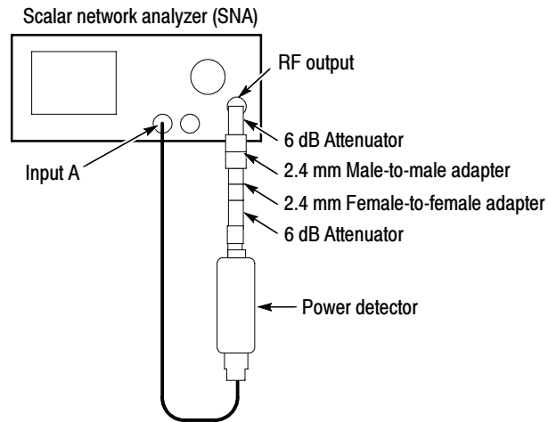
Figure 2-35: Adapter-loss hookup
