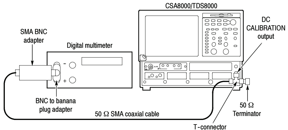
Figure 2-23: Hookup for DC calibration test
