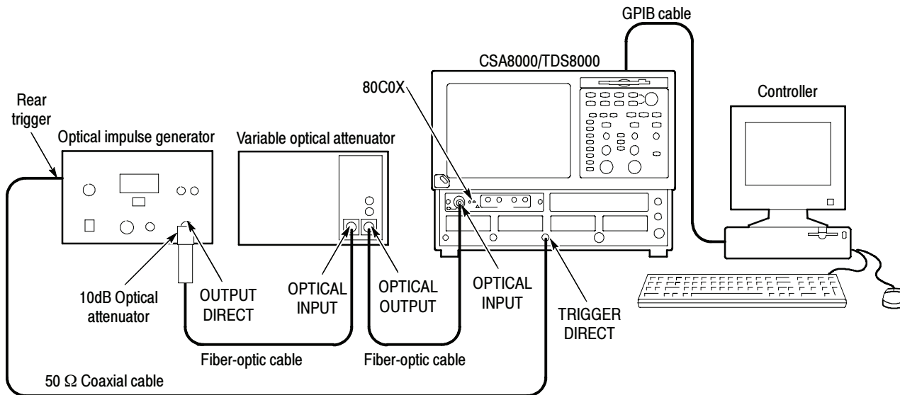
Figure 2- 45: Minimum optical bandwidth and reference receiver frequency response hookup
