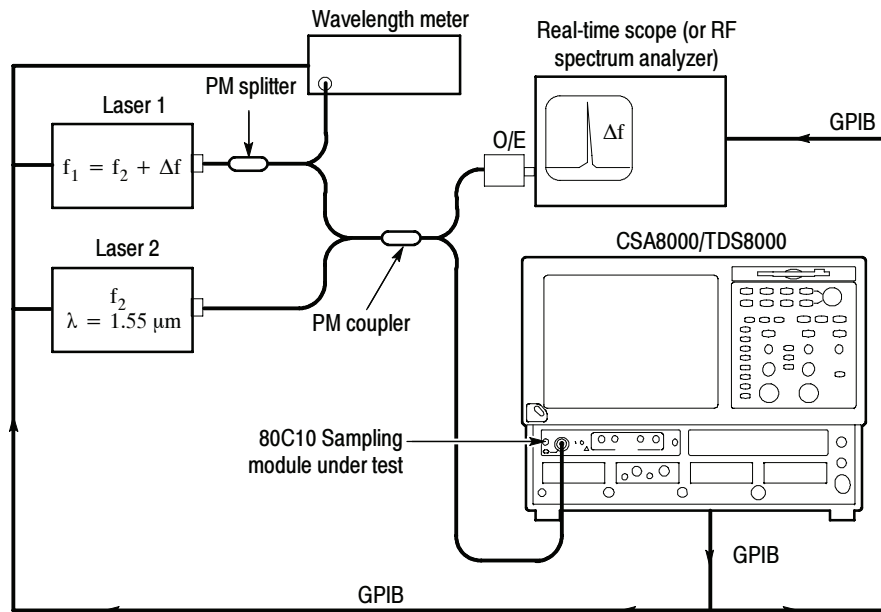
Figure 2- 47: Hookup for heterodyne test
