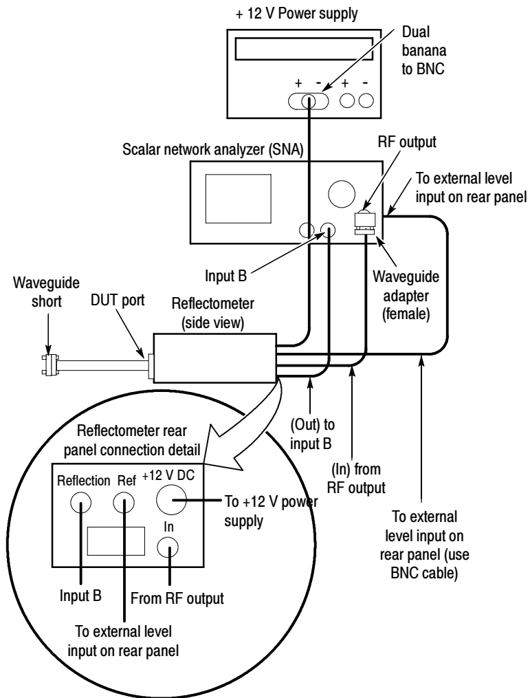
Figure 2-37: SNA/Waveguide Characterization
