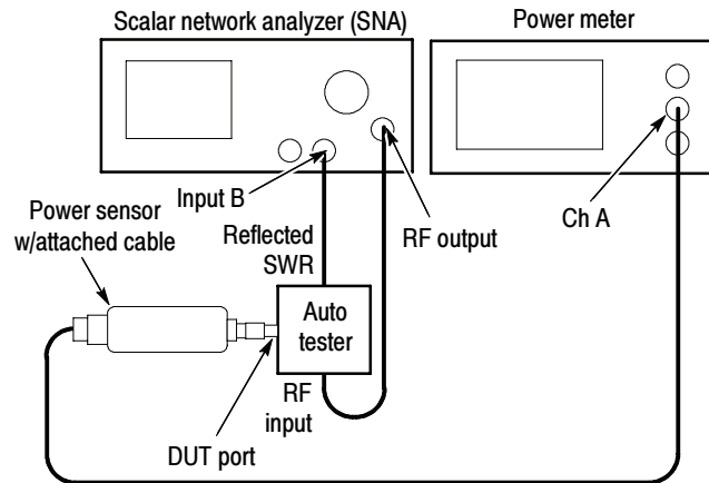
Figure 2-33: Hookup to measure Power in
