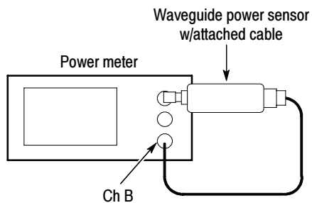
Figure 2-38: Power-reference characterization hookup
